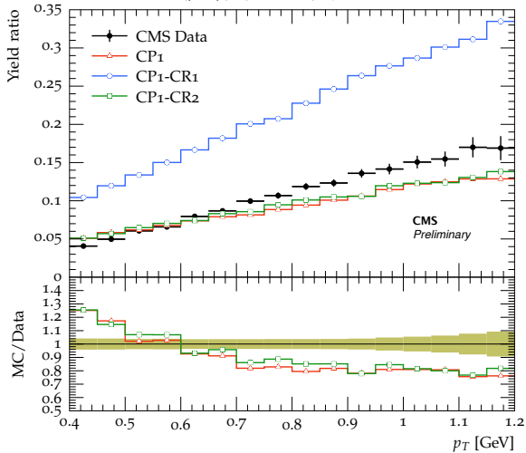
Minimum Bias, (p + \bar{p})/(\pi^+ + \pi^-) , \sqrt{s} = 13 TeV
