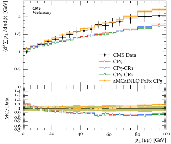
Z \rightarrow \mu^+ \mu^- , Transverse region, \sqrt{s} = 13 TeV
