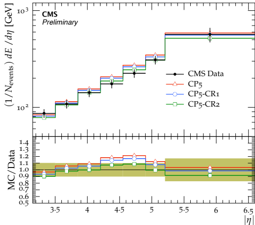
Energy flow, inclusive selection, \sqrt{s} = 13 TeV
