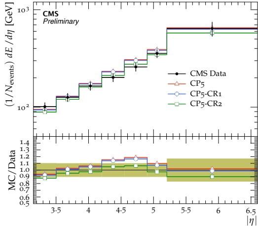
Energy flow, NSD selection, \sqrt{s} = 13 TeV
