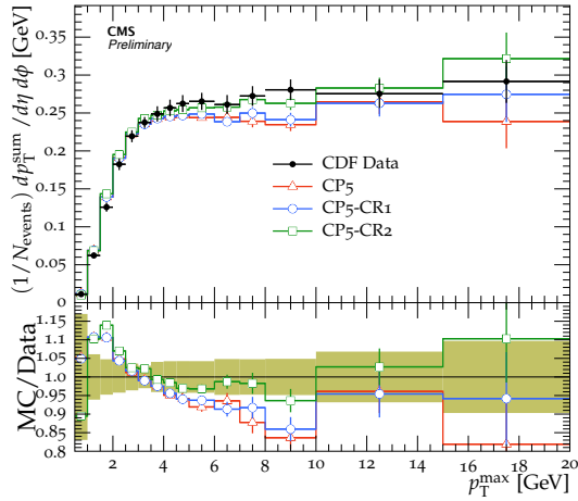
TransMAX charged p_{\text{T}}^{\text{sum}} density, \sqrt{s} = 1.96 TeV
