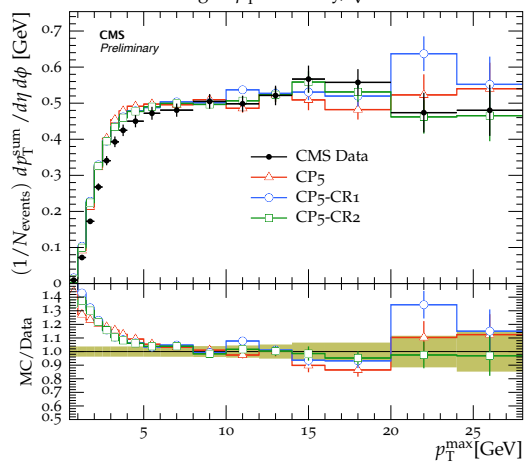
TransMAX charged p_{\text{T}}^{\text{sum}} density, \sqrt{s} = 7 TeV
