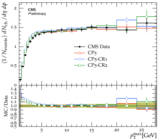
TransMAX charged-particle density, \sqrt{s} = 7 TeV
