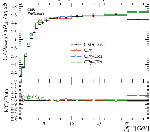
TransMAX charged-particle density, \sqrt{s} = 13 TeV
