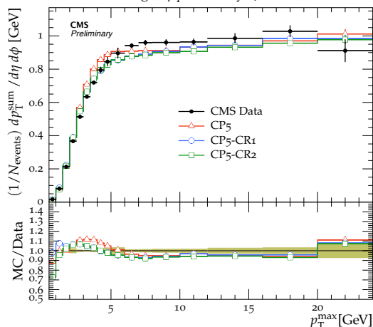
TransMAX charged p_T^{\text{sum}} density, \sqrt{s} = 13 TeV
