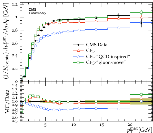
TransMAX charged p_{\text{T}}^{\text{sum}} density, \sqrt{s} = 13 TeV
