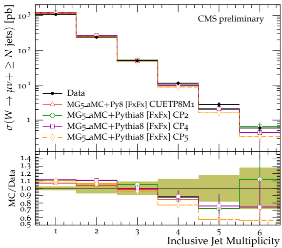
Inclusive Jet Multiplicity \sqrt{s} = 13 TeV
