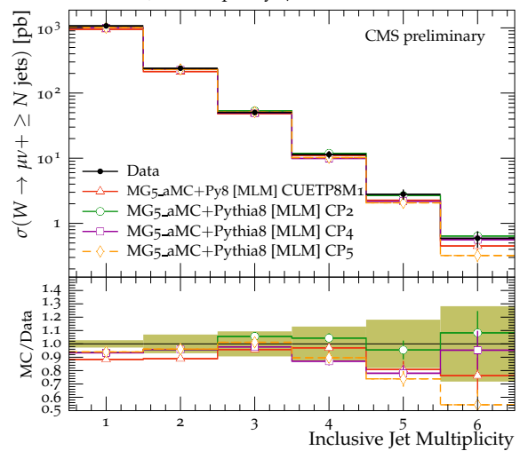
Inclusive Jet Multiplicity \sqrt{s} = 13 TeV
