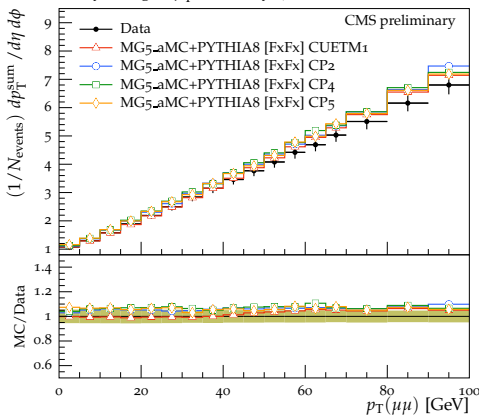
Away charged p_T^{\text{sum}} density \sqrt{s} = 13 TeV
