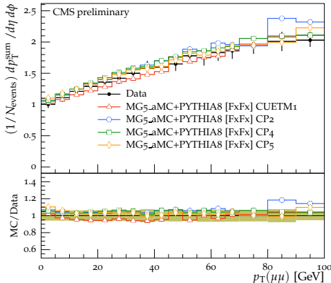
Away charged p_T^{\text{sum}} density \sqrt{s} = 13 TeV
