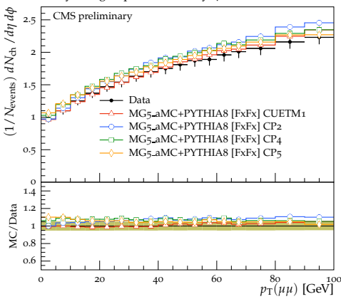
Away charged-particle density \sqrt{s} = 13 TeV
