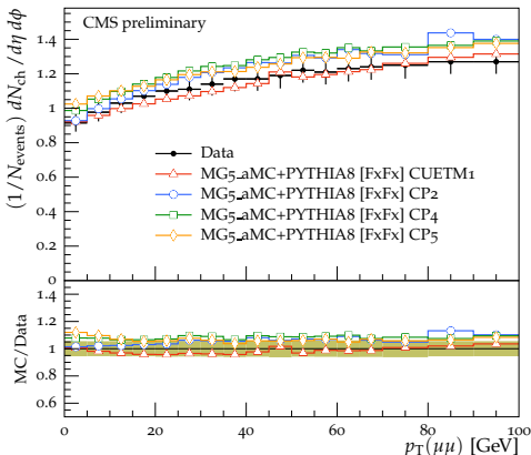
Away charged-particle density \sqrt{s} = 13 TeV
