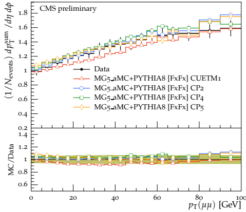
Transverse charged p_T^{\text{sum}} density \sqrt{s} = 13 TeV
