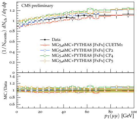
Transverse charged-particle density \sqrt{s} = 13 TeV
