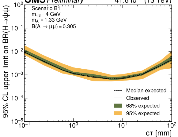
CMS Preliminary 41.6 fb -1 (13 TeV)
