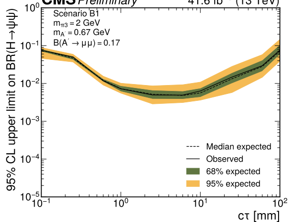
CMS Preliminary 41.6 fb -1 (13 TeV)
