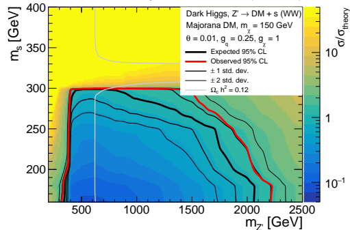
CMS Preliminary 137 fb -1 (13 TeV)
