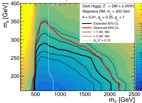
CMS Preliminary 137 fb -1 (13 TeV)
