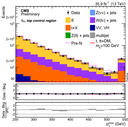
(a) AH1m- \bar{t}\bar{t}
