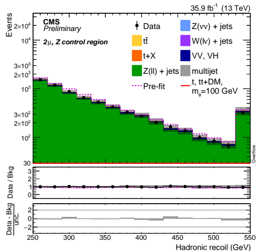
(f) AH2 \mu -Z
