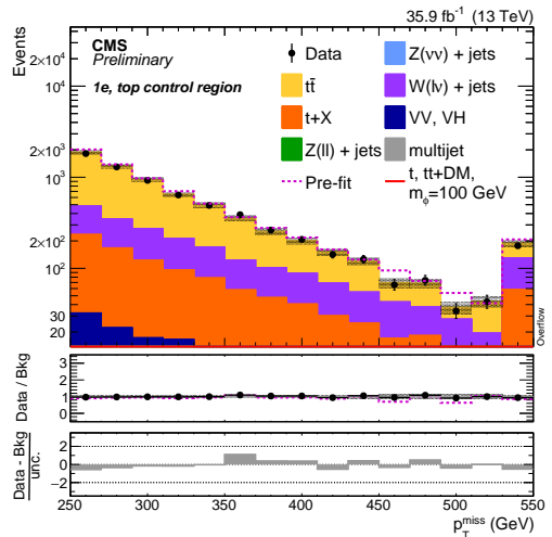
(b) AH1e- \bar{t}\bar{t}
