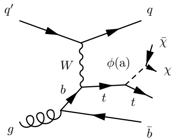
(b) t/\bar{t} + \text{DM, t-channel}
