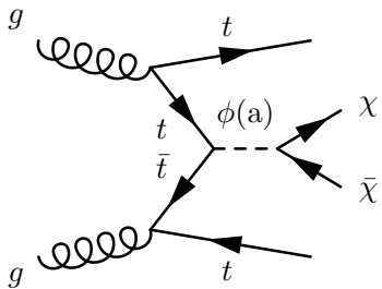
(a) t\bar{t} + \text{DM}
