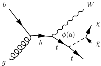
(c) t/\bar{t} + \text{DM, tW-channel}
