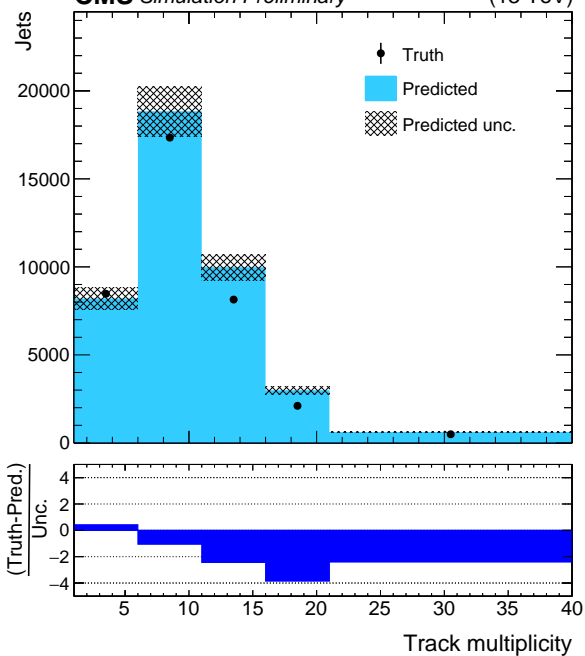
CMS Simulation Preliminary (13 TeV)
