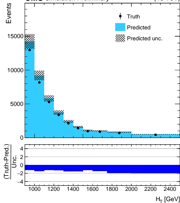
CMS Simulation Preliminary (13 TeV)
