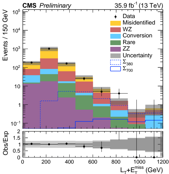
(c) L_T + E_T^{\text{miss}} , L3BelowZ
