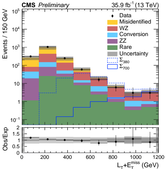
(b) L_T + E_T^{\text{miss}} , L3AboveZ
