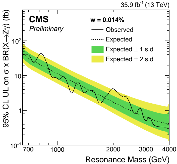
(a) \frac{\Gamma}{m} = 0.014\% : combined limit
