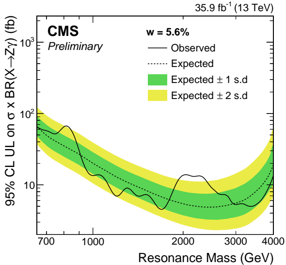
(b) \frac{\Gamma}{m} = 5.6\% : combined limit
