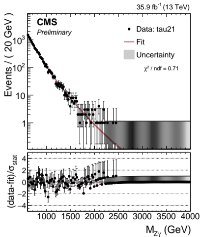
(b) tau21 SR
