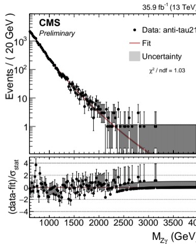
(c) anti-tau21 SR
