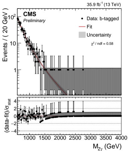
(a) b-tagged SR
