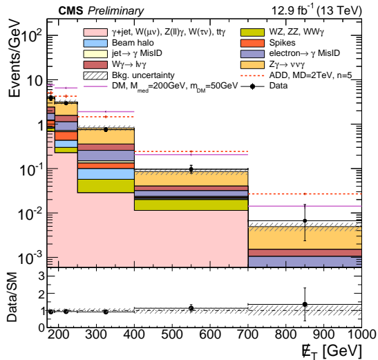
(b) Particle Flow E_T
