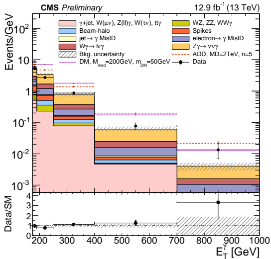
(a) Photon p_T
