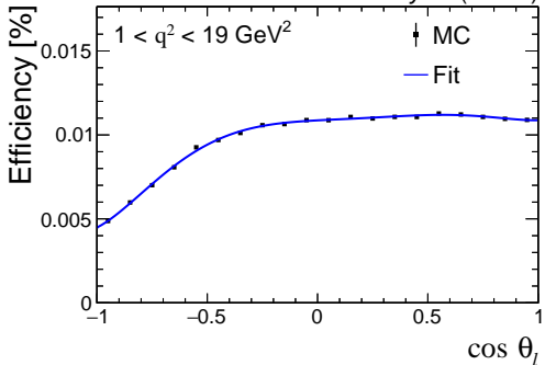
CMS Simulation Preliminary (8 TeV)
