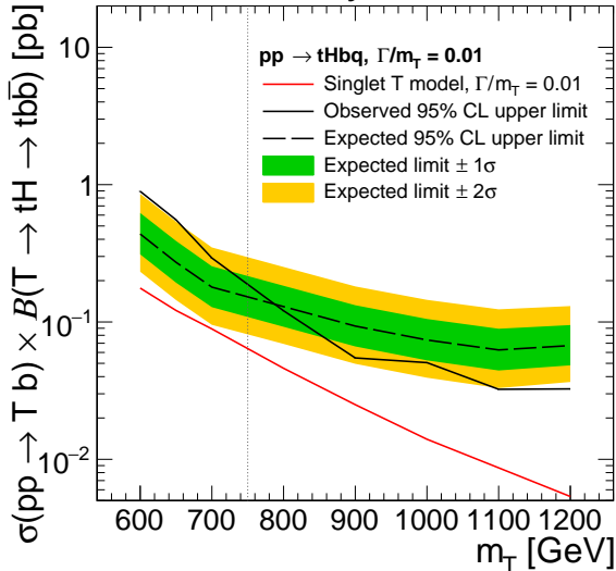
CMS Preliminary 138 fb -1 (13 TeV)
