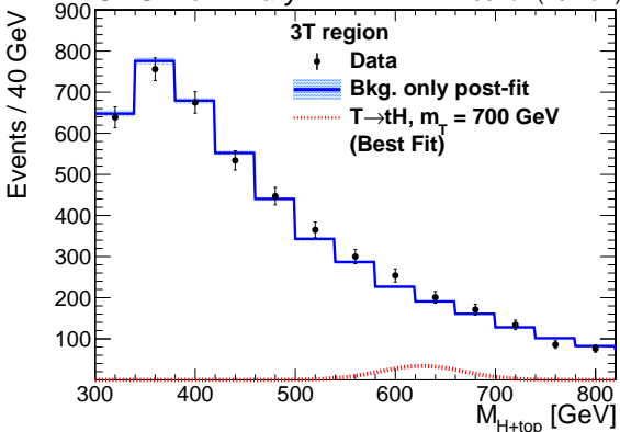
CMS Preliminary 138 fb -1 (13 TeV)
