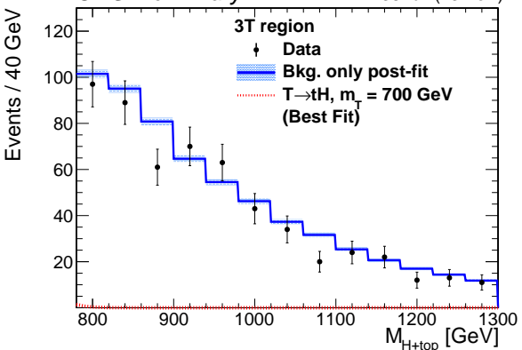
CMS Preliminary 138 fb -1 (13 TeV)
