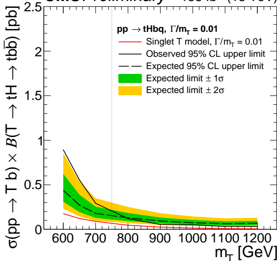
CMS Preliminary 138 fb -1 (13 TeV)
