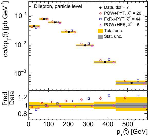
CMS 138 \text{ fb}^{-1} (13 \text{ TeV})
