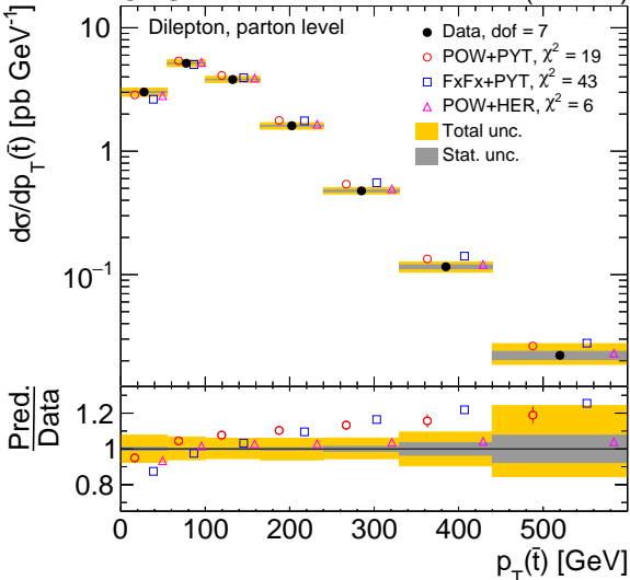
CMS 138 \text{ fb}^{-1} (13 \text{ TeV})
