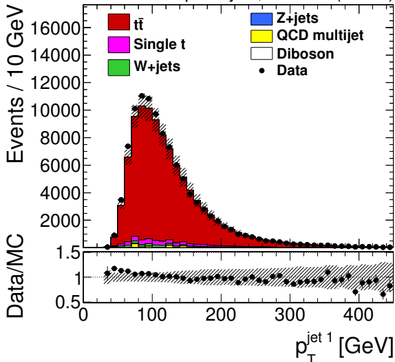
CMS Lepton+jets, 19.7 fb -1 (8 TeV)
