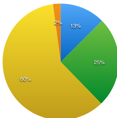
Anti-tagged Region in Mass Sideband
