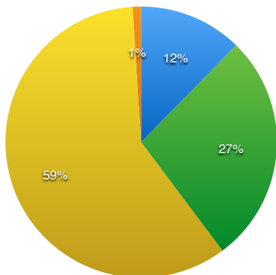
Anti-tagged Region Mass [85,135]GeV
