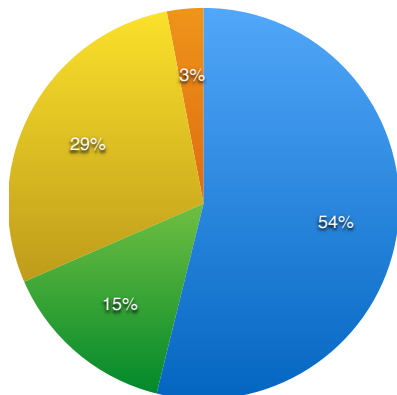
Double Higgs Tag
