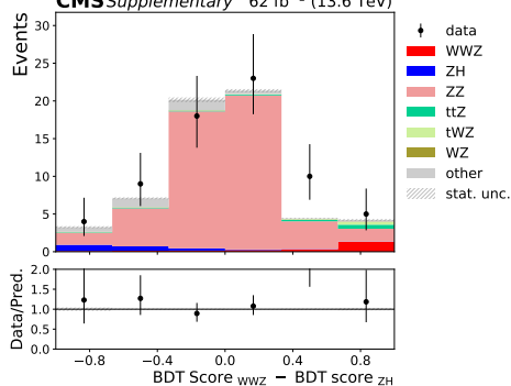
CMS Supplementary 62 fb -1 (13.6 TeV)
