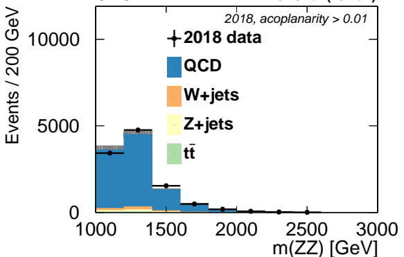
CMS 52.9 fb -1 (13 TeV)
