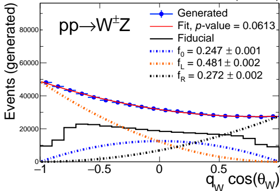
CMS Simulation 137 fb -1 (13 TeV)
