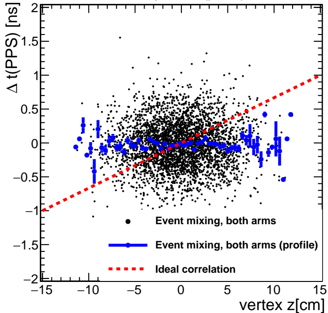
CMS Preliminary 2018 ( \mu \approx 1 )
