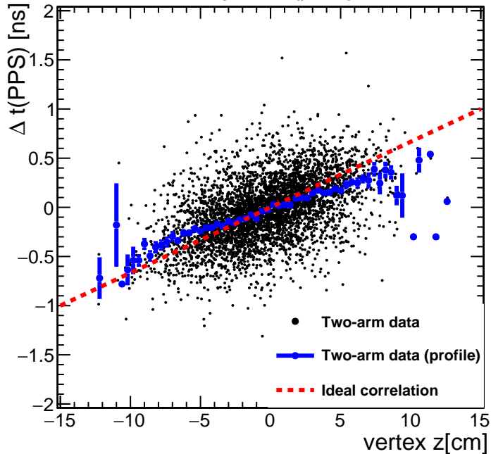
CMS Preliminary 2018 ( \mu \approx 1 )
