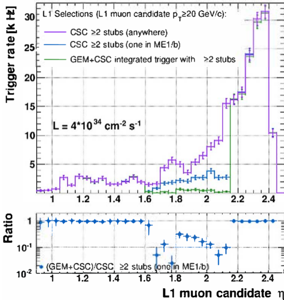
CMS Simulation
