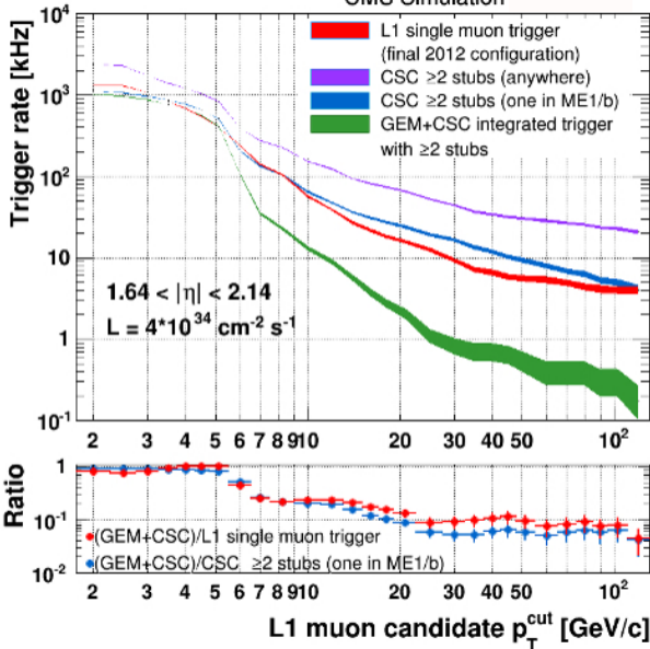
CMS Simulation
