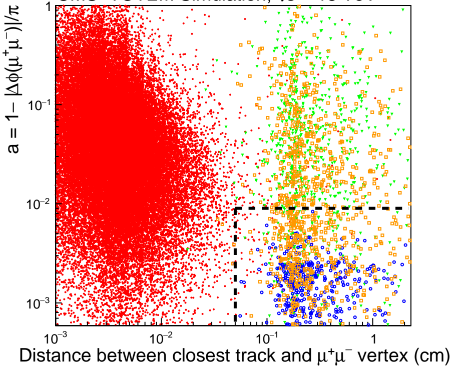
CMS+TOTEM Simulation, \sqrt{s} = 13 TeV
