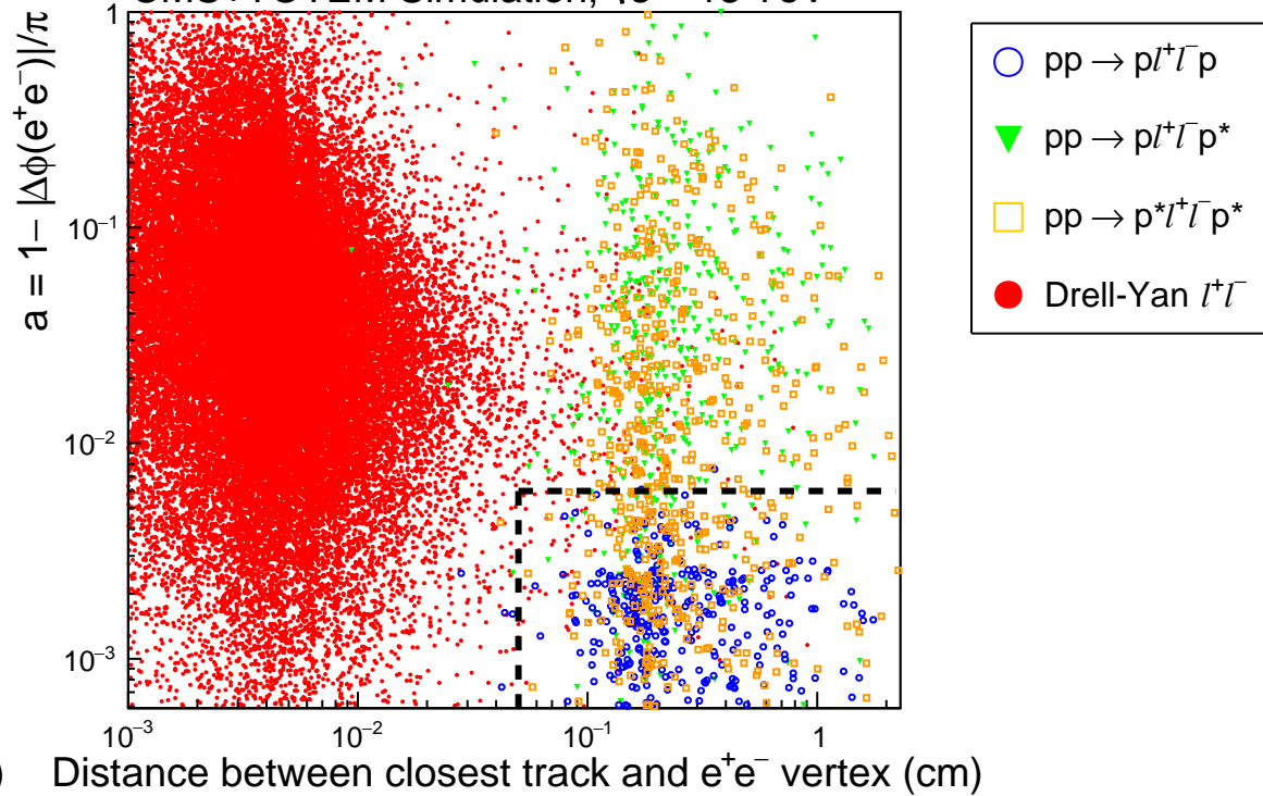
CMS+TOTEM Simulation, \sqrt{s} = 13 TeV
