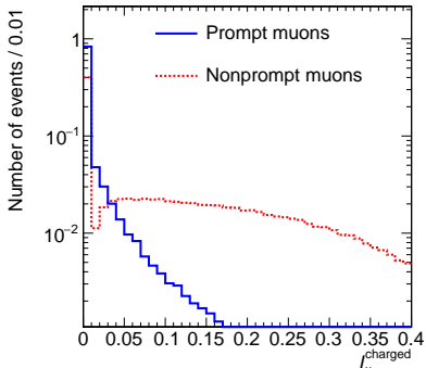
CMS Simulation (13 TeV)
