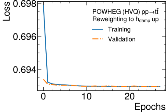
CMS Simulation
