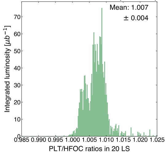
CMS PbPb 2018 (5.02 TeV)
