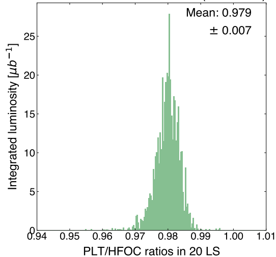
CMS PbPb 2015 (5.02 TeV)
