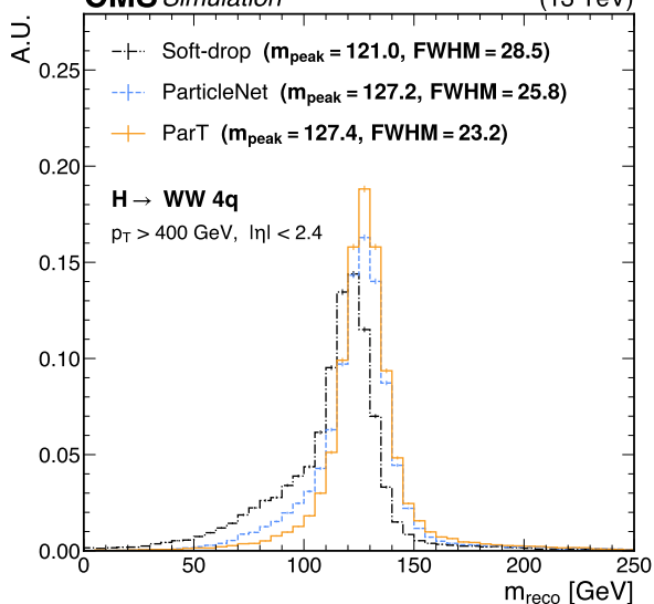
CMS Simulation (13 TeV)
