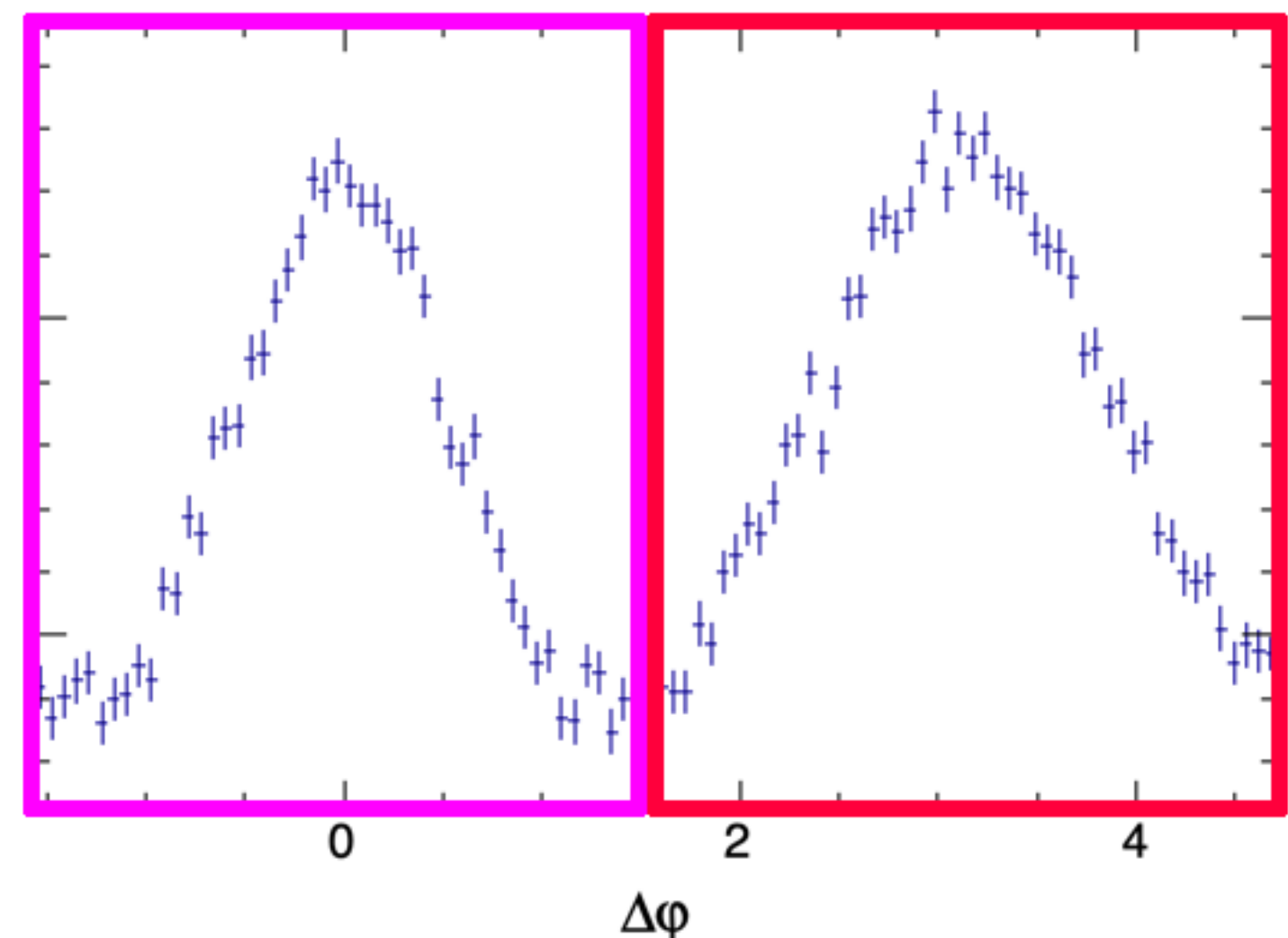
Long-range correlation
