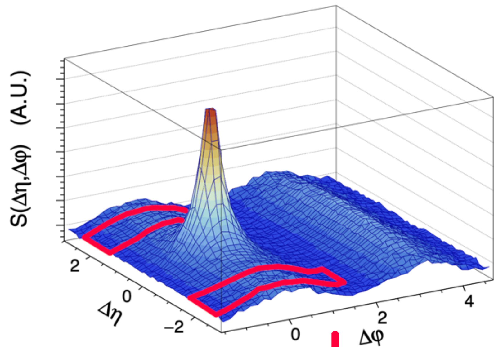
Subleading jet-hadron correlation
