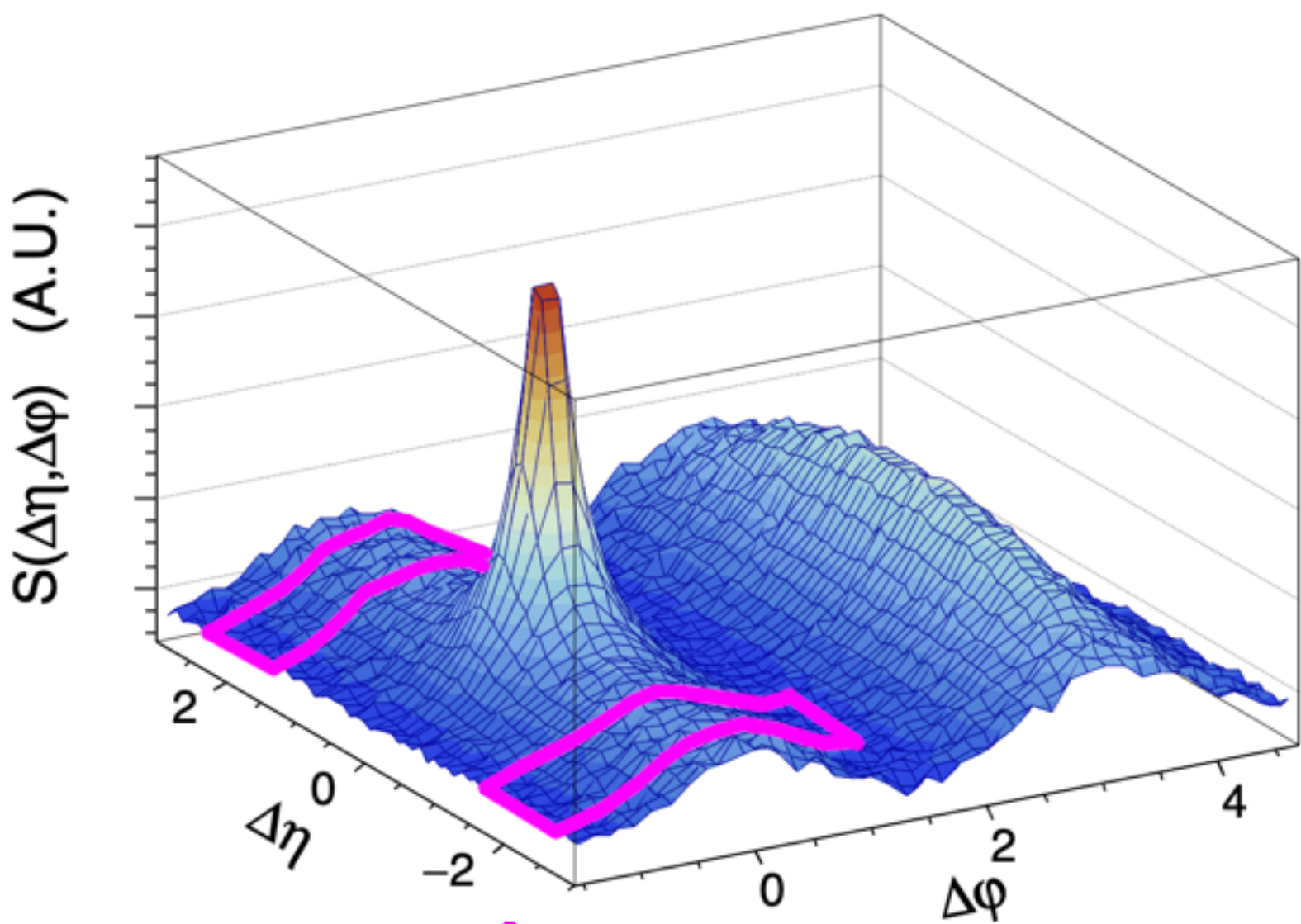
Leading jet-hadron correlation
