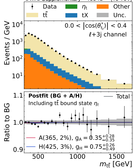
CMS Supplementary 138 fb -1 (13 TeV)
