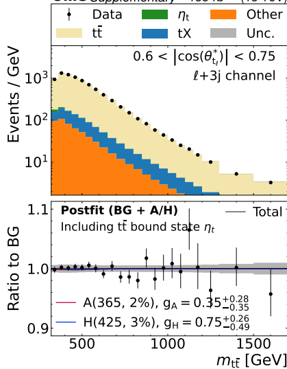
CMS Supplementary 138 fb -1 (13 TeV)
