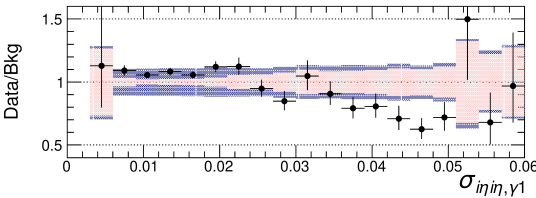
CMS 138 fb -1 (13 TeV)
