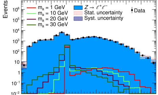
CMS 138 fb -1 (13 TeV)
