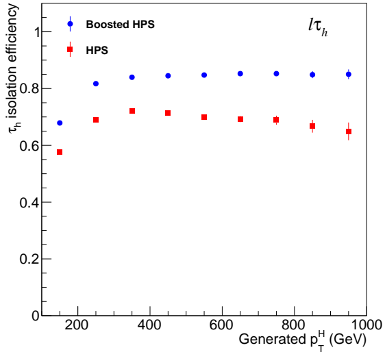
CMS Simulation
