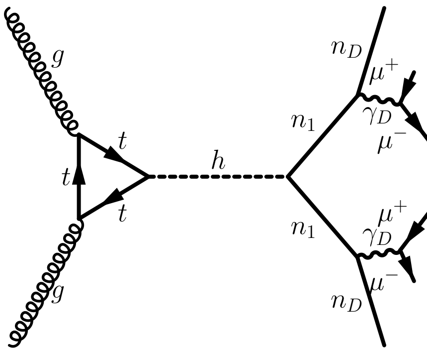
Dark SUSY
