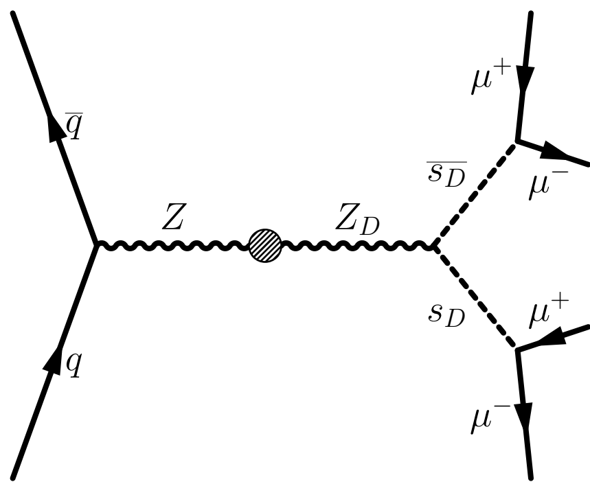
Vector Portal
