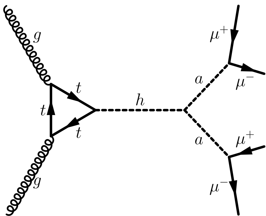
ALP
