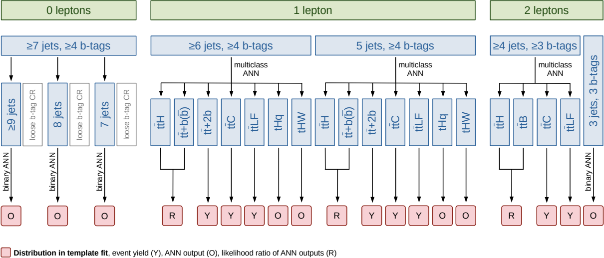
Legend: █ Distribution in template fit, event yield (Y), ANN output (O), likelihood ratio of ANN outputs (R)
