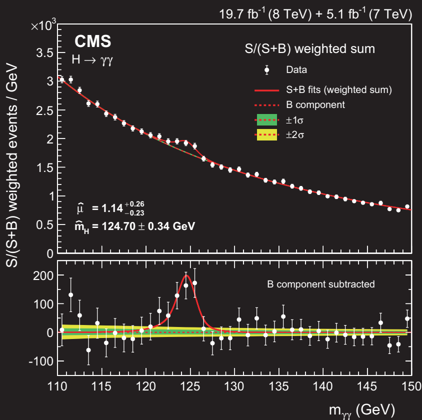
Diphoton mass spectrum weighted by the ratio S/(S+B) in each event class (upper plot), together with the background subtracted weighted mass spectrum (lower plot). From The CMS Collaboration: Observation of the diphoton decay of the Higgs boson and measurement of its properties.
