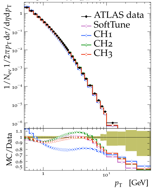
Charged particle p_T , N_{ch} \geq 6 , \sqrt{s} = 7 TeV
