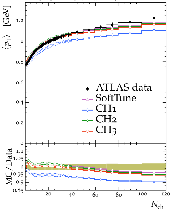
Charged particle \langle p_T \rangle , N_{ch} \geq 1 , \sqrt{s} = 7 TeV
