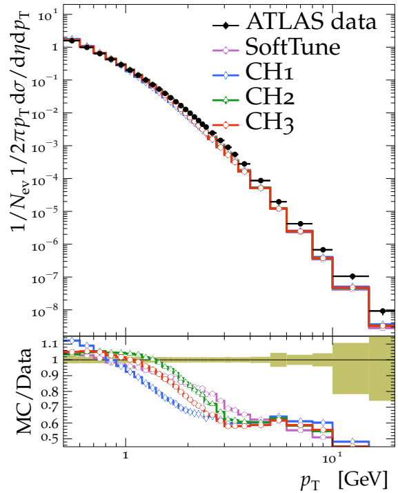
Charged particle p_T , N_{ch} \geq 6 , \sqrt{s} = 0.9 TeV
