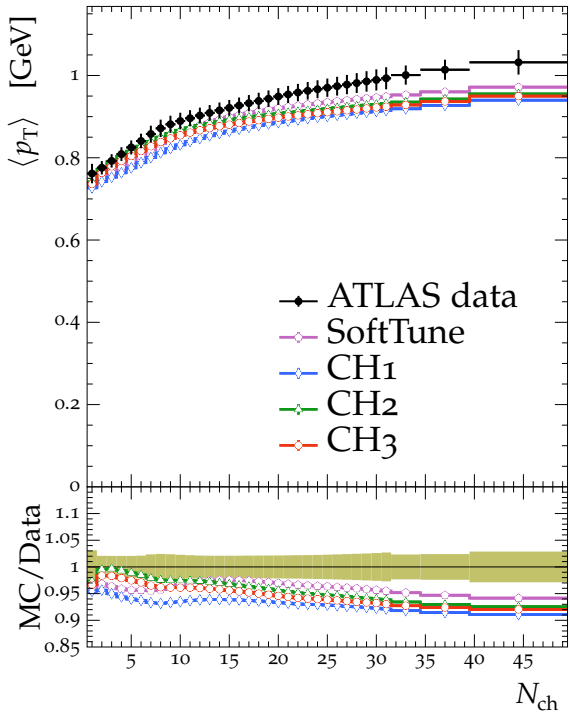
Charged particle \langle p_T \rangle , N_{ch} \geq 1 , \sqrt{s} = 0.9 TeV
