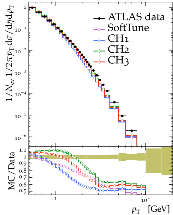
Charged particle p_T , N_{ch} \geq 1 , \sqrt{s} = 0.9 TeV
