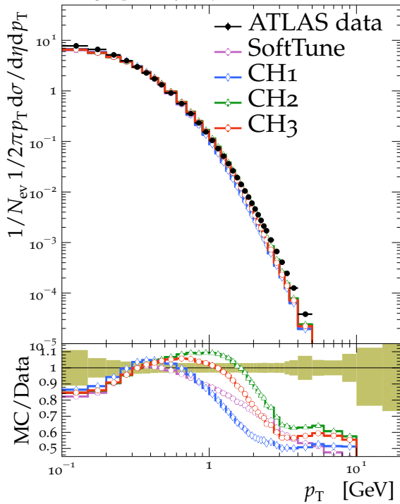
Charged particle p_T , N_{ch} \geq 2 , \sqrt{s} = 0.9 TeV
