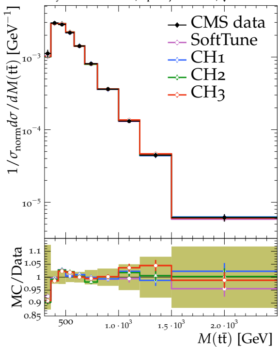
t\bar{t} system invariant mass, lepton+jets t\bar{t} events, \sqrt{s} = 13 TeV
