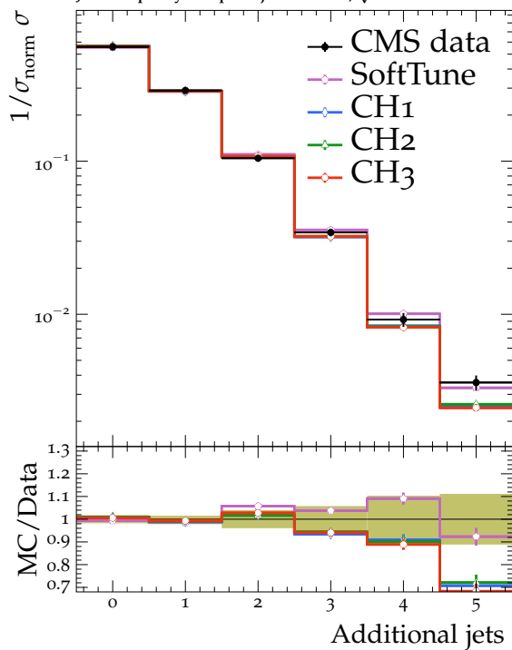
Jet multiplicity in lepton+jets t\bar{t} events, \sqrt{s} = 13 TeV
