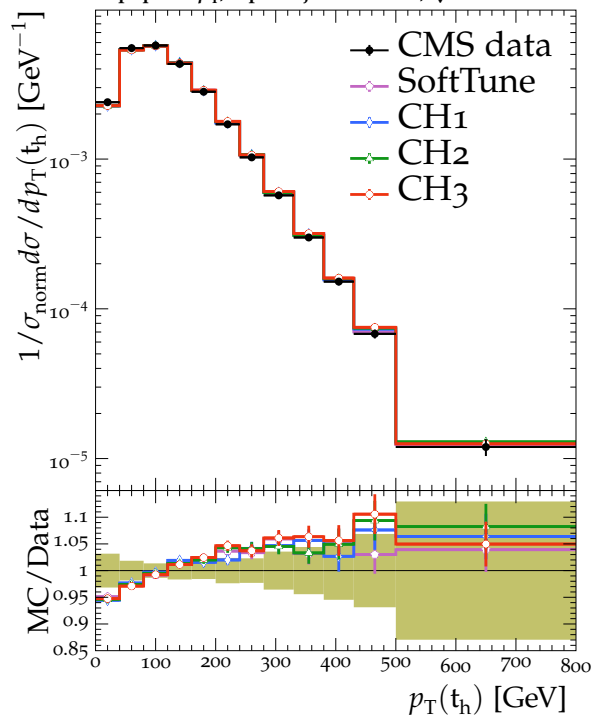
Top quark p_T , lepton+jets t\bar{t} events, \sqrt{s} = 13 TeV
