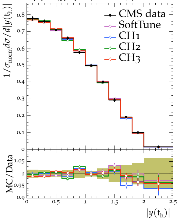
Top quark |y| , lepton+jets t\bar{t} events, \sqrt{s} = 13 TeV
