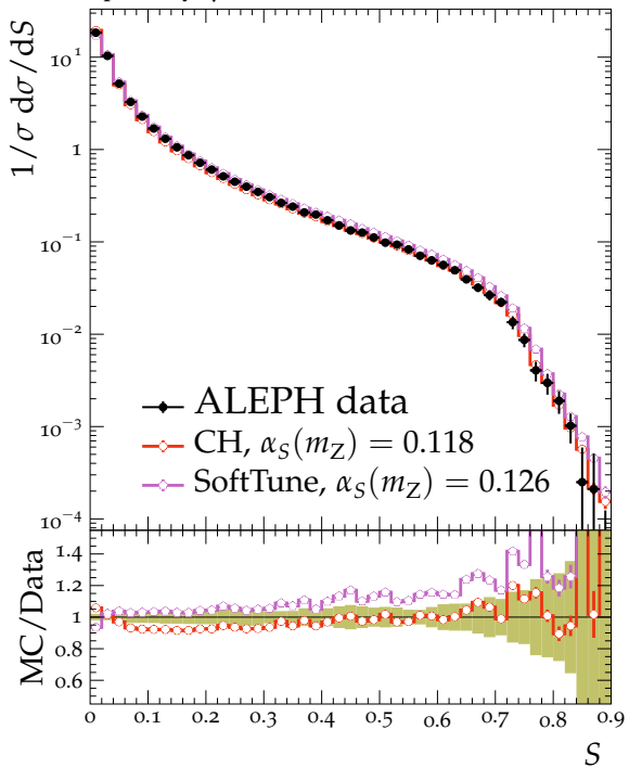
Sphericity, \sqrt{s} = 91.2 GeV
