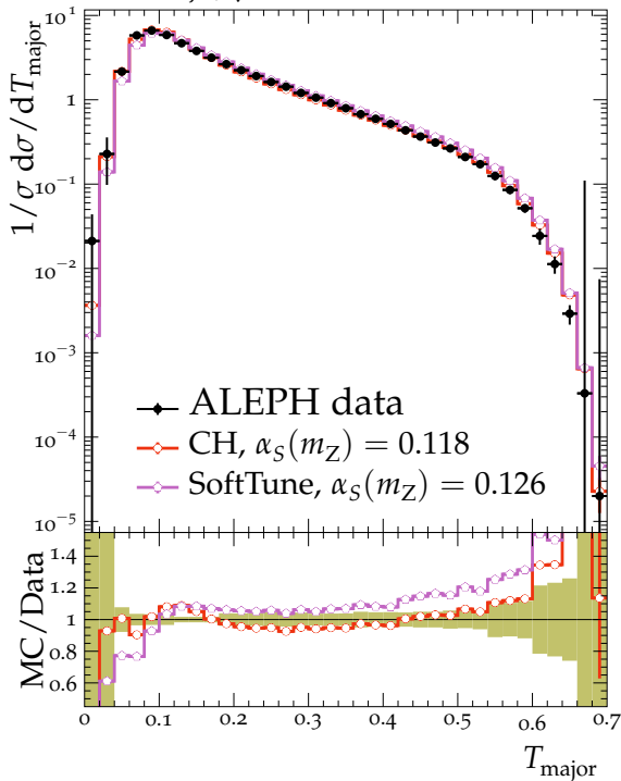
Thrust major, \sqrt{s} = 91.2 GeV
