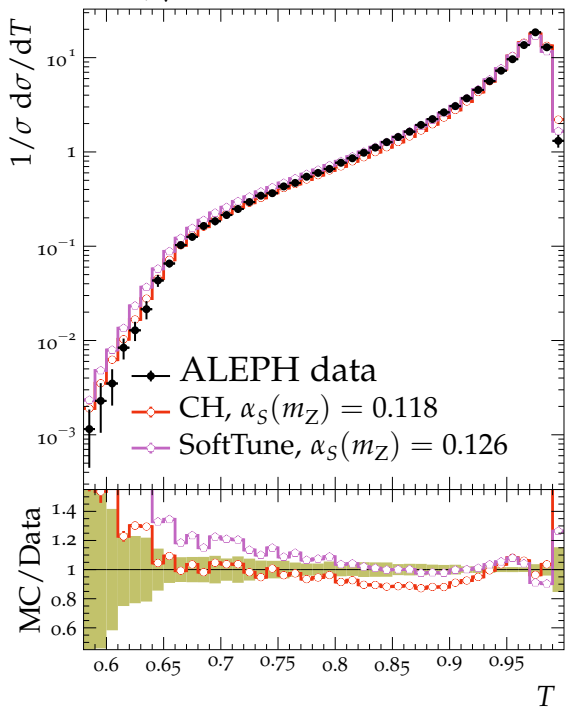
Thrust, \sqrt{s} = 91.2 GeV
