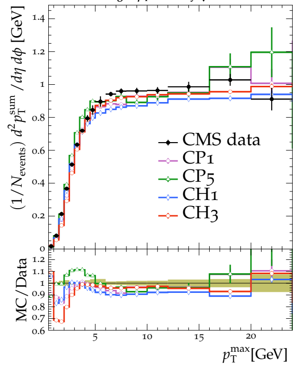
TransMin charged-particle density \sqrt{s} = 13 TeV
