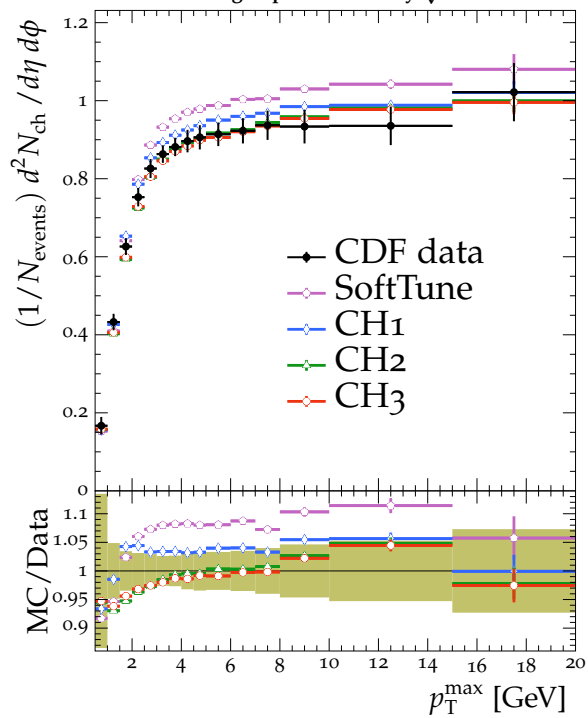
TransMax charged-particle density \sqrt{s} = 1.96 TeV
