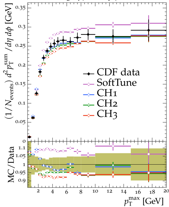
TransMin charged-particle density \sqrt{s} = 1.96 TeV
