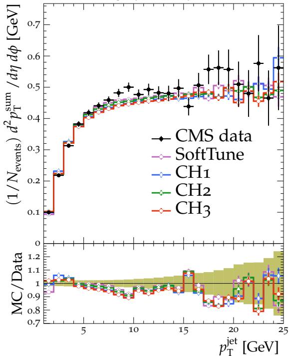
Transverse charged p_T^{\text{sum}} density \sqrt{s} = 0.9 TeV
