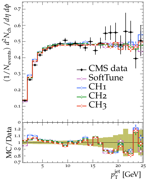
Transverse charged-particle density \sqrt{s} = 0.9 TeV
