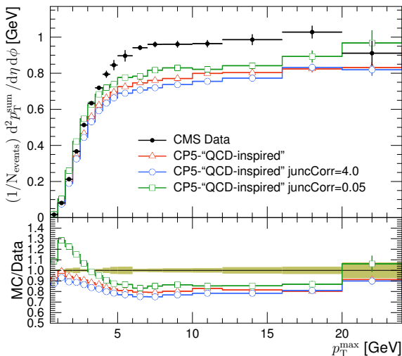
TransMAX charged p_{\text{T}}^{\text{sum}} density \sqrt{s} = 13 TeV
